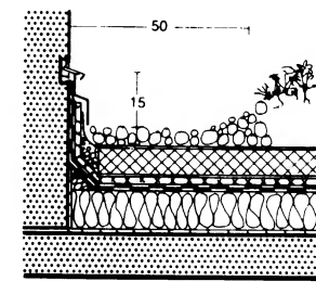
⑭ Wall connection with shingle edging strip
